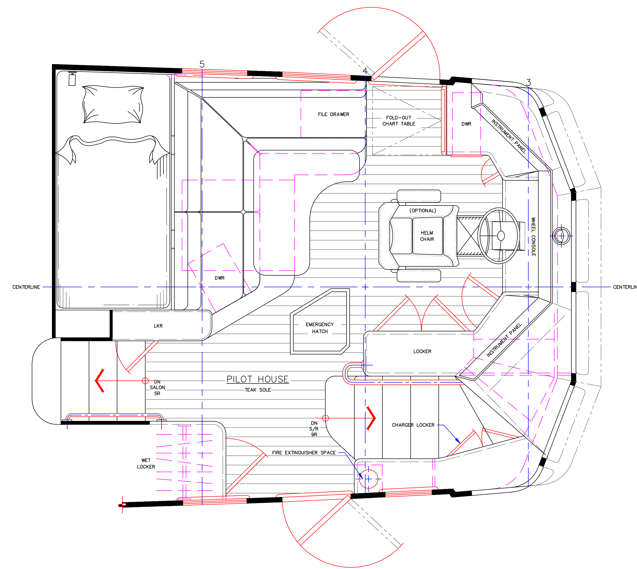
PILOT HOUSE PLAN
