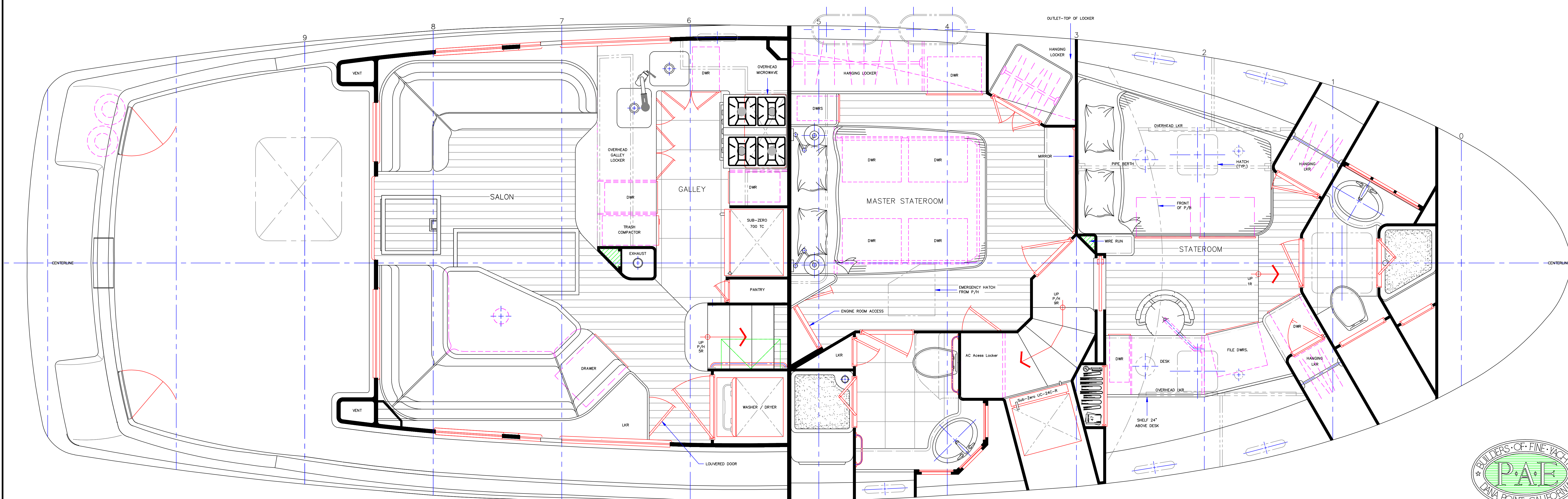
PILOT HOUSE PLAN
