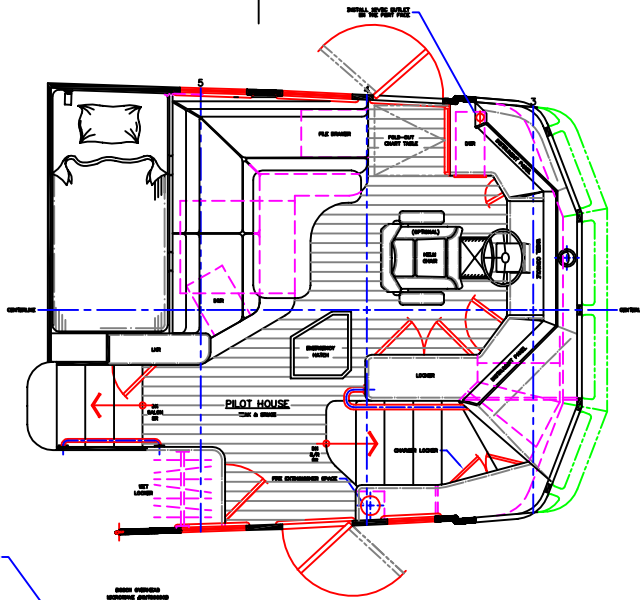
PILOT HOUSE PLAN
