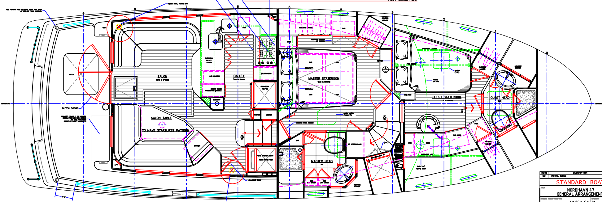
GENERAL ARRANGEMENT
