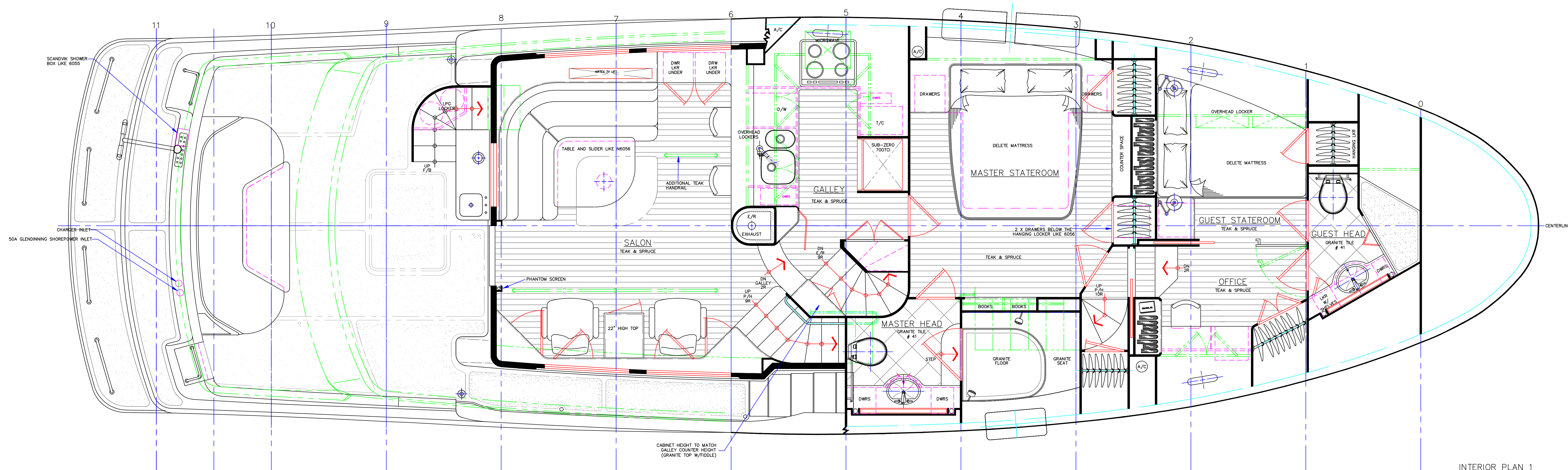
INTERIOR PLAN 1
