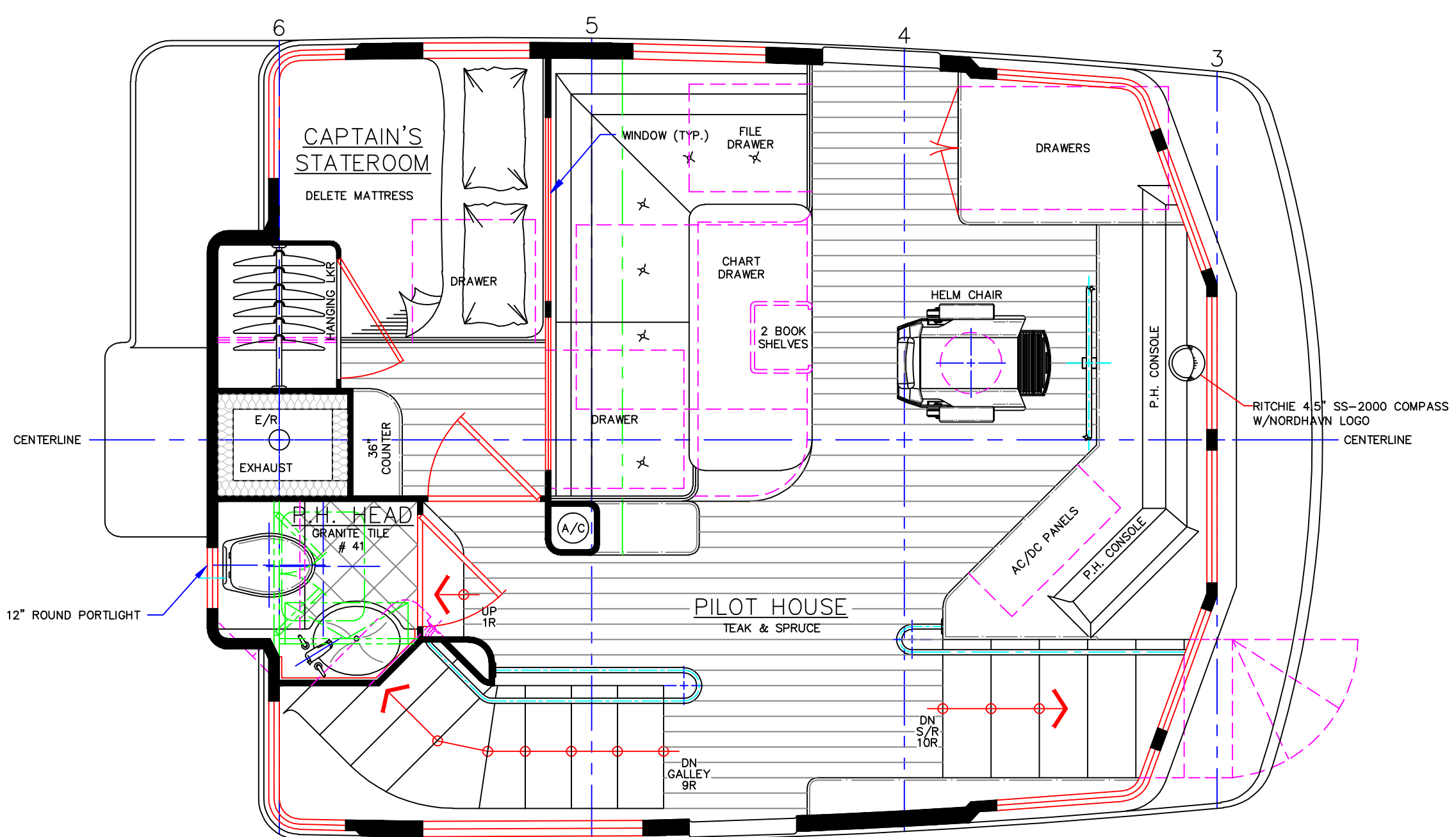
PILOT HOUSE PLAN
