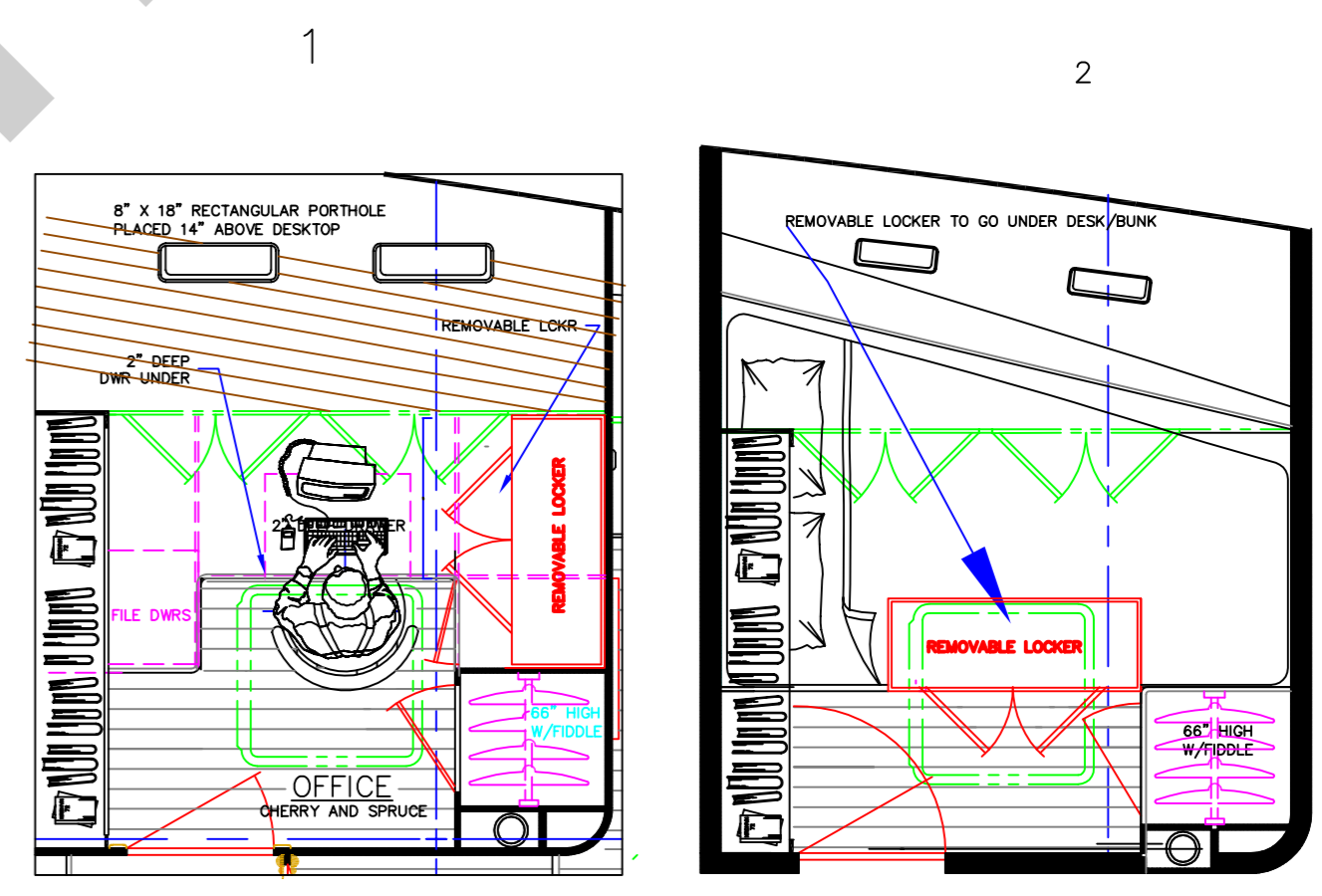
PORT OFFICE BERTH PLAN VEIW 1/2"=1'-0"
