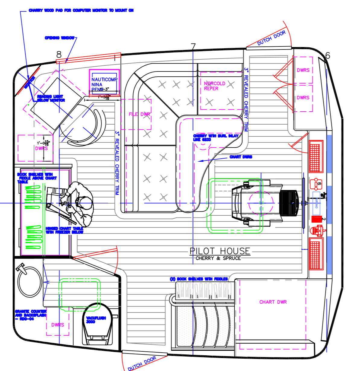
PILOT HOUSE 1/2"=1'-0"
