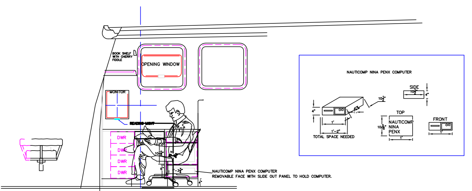
PILOT HOUSE PORT PROFILE 1/2"=1'-0"
