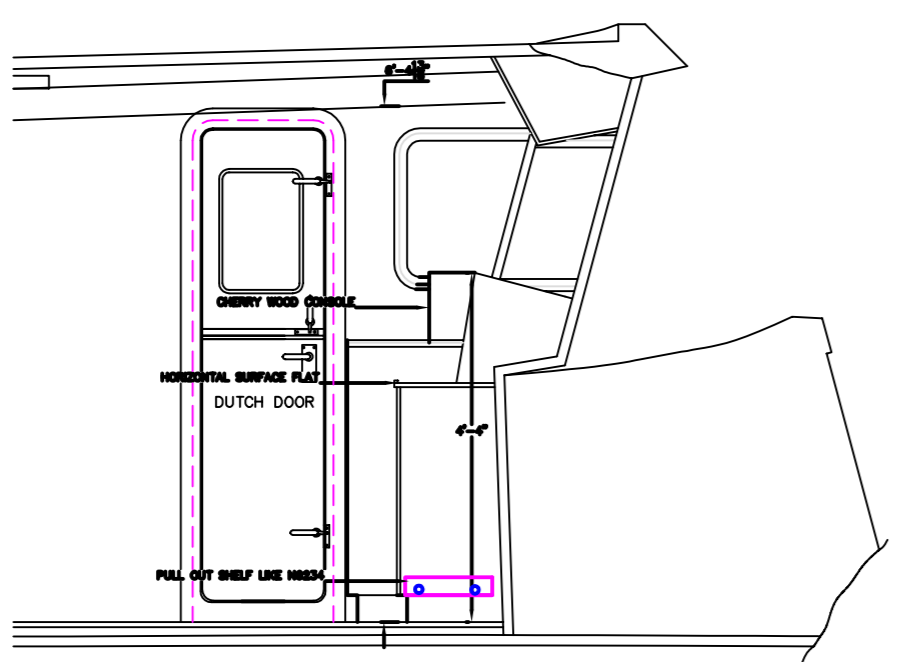
PILOT HOUSE PORT PROFILE 1/2"=1'-0"
