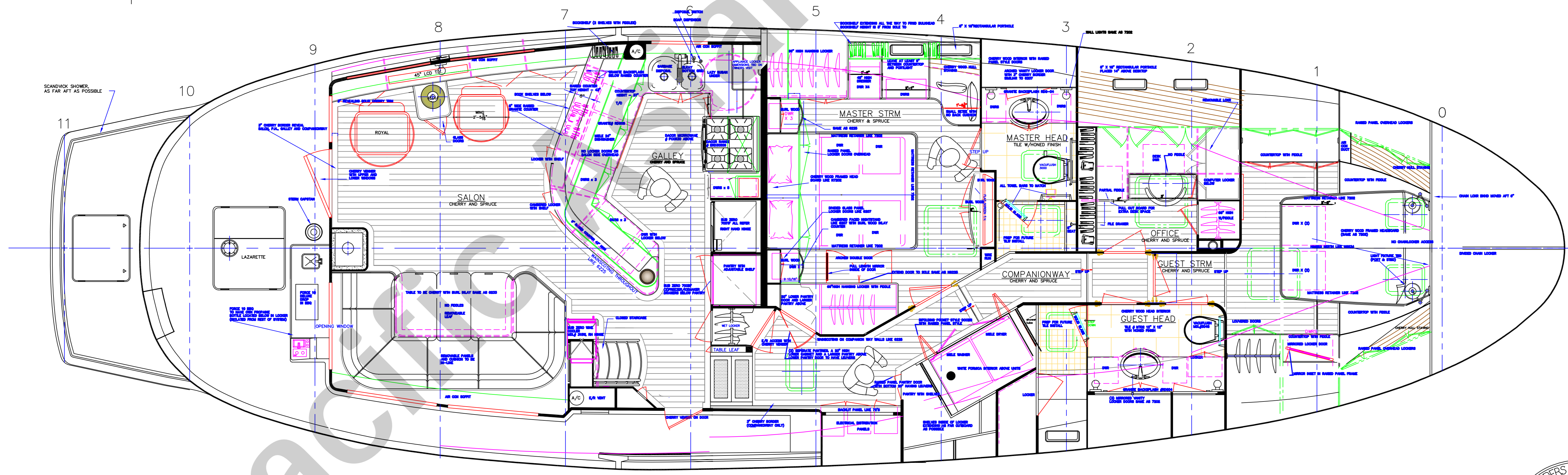
INTERIOR LAYOUT 1/2"=1'-0"
