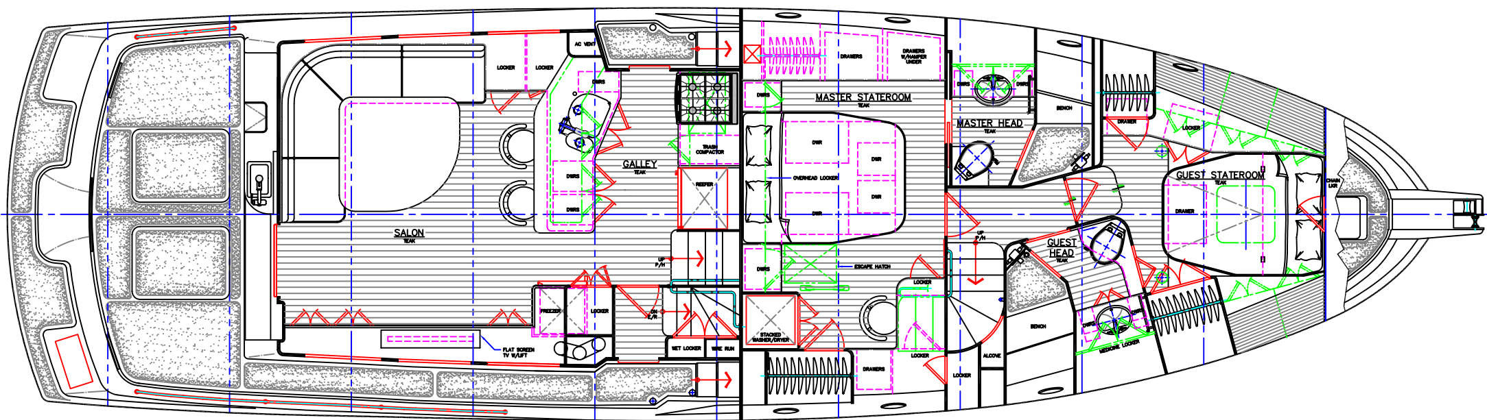
INTERIOR PLAN 1/2"=1'-0"
