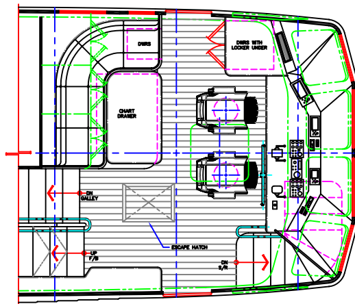
PILOT HOUSE 1/2"=1'-0"
