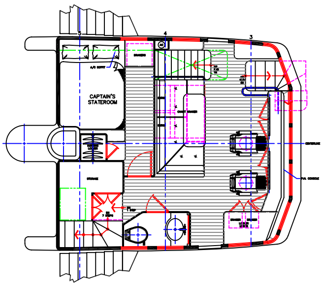
PILOT HOUSE PLAN 1/8"=1'-0"
