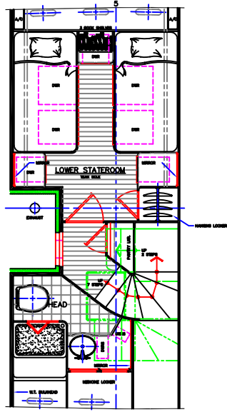
INTERIOR PLAN (LOWER DECK) 1/8"=1'-0"
