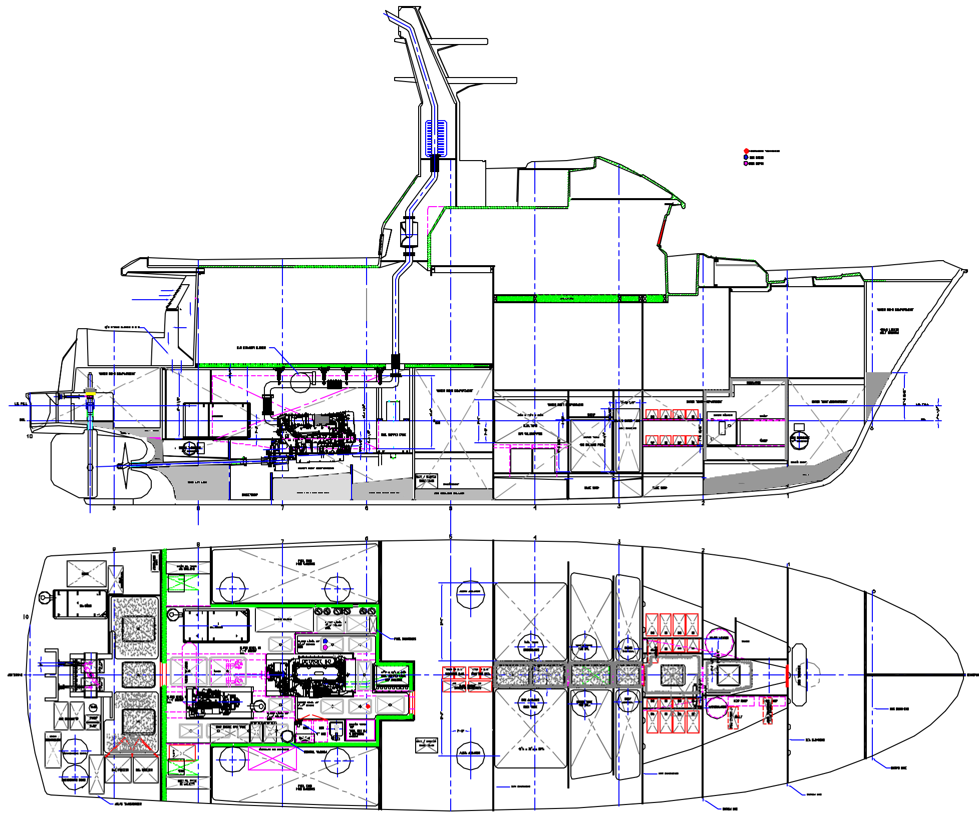
MACHINERY AND TANKAGE PLAN
