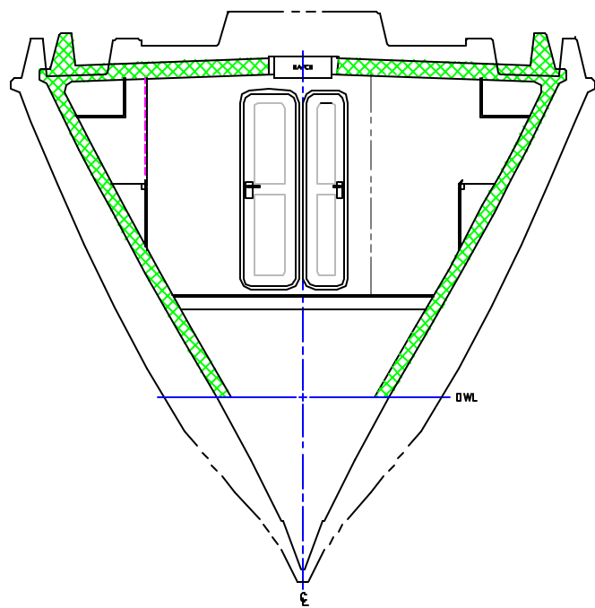
SECTION @ STATION 1 LOOKING AFT 1/2"=1'-0"
