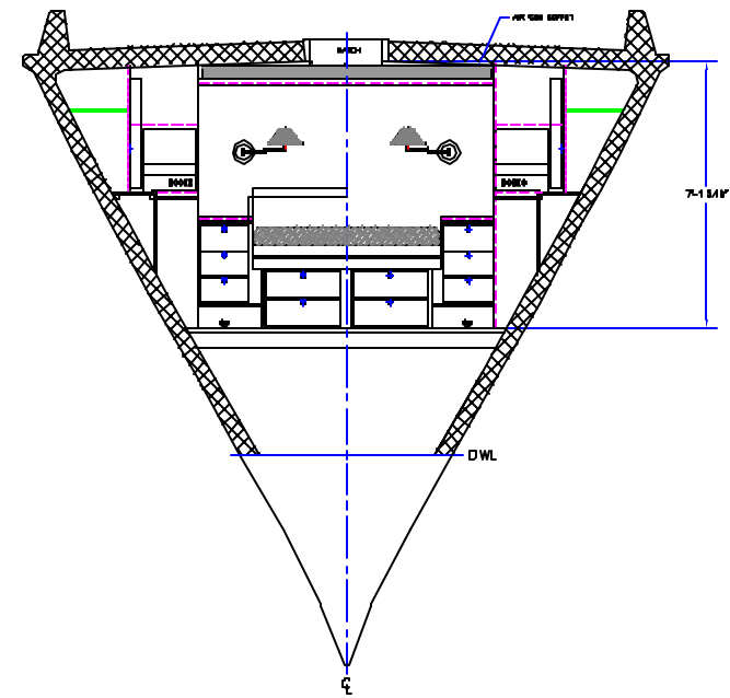
SECTION @ STATION 1 LOOKING FWD 1/8\"/>
