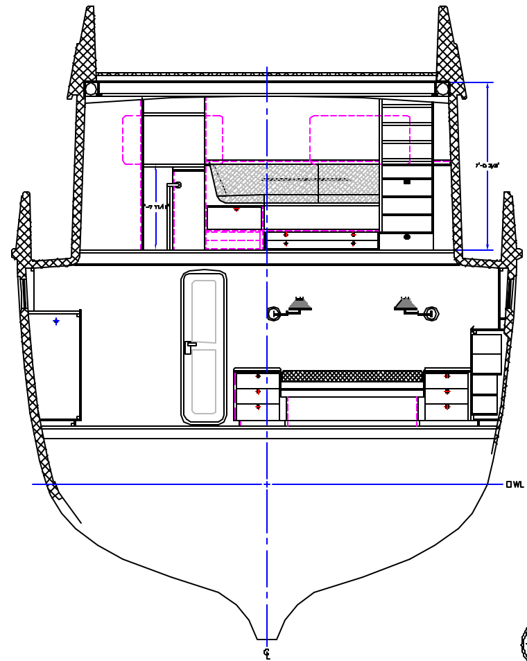
SECTION @ STATION 3.5 LOOKING AFT 1/2\"/>
