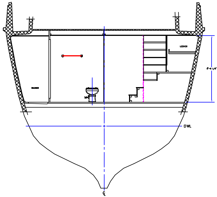
SECTION @ STATION 2.75 LOOKING AFT 1/2\"/>
