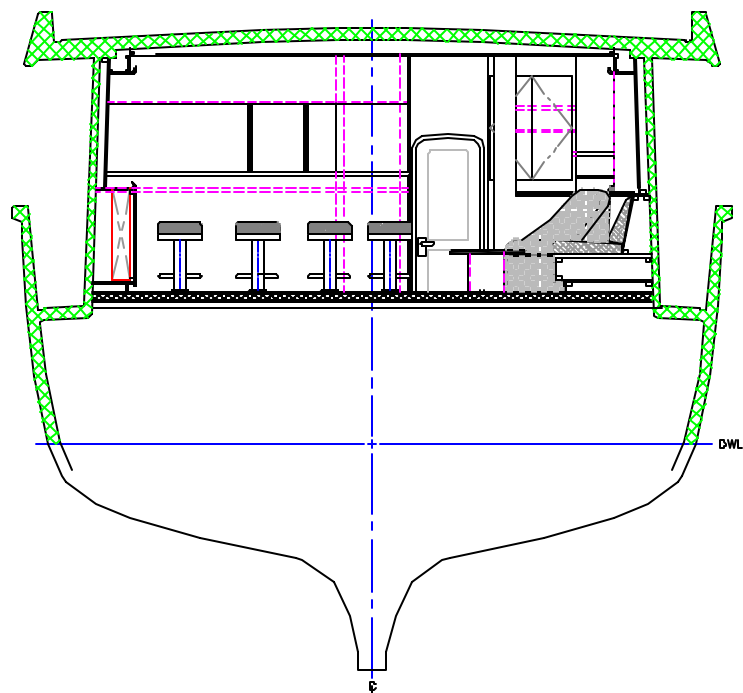
SECTION @ STATION 7 LOOKING FWD 1/2"=1'-0"
