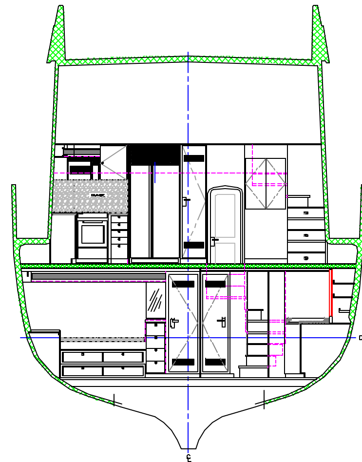
STATION 5 LOOKING FWD 1/2"=1'-0"
