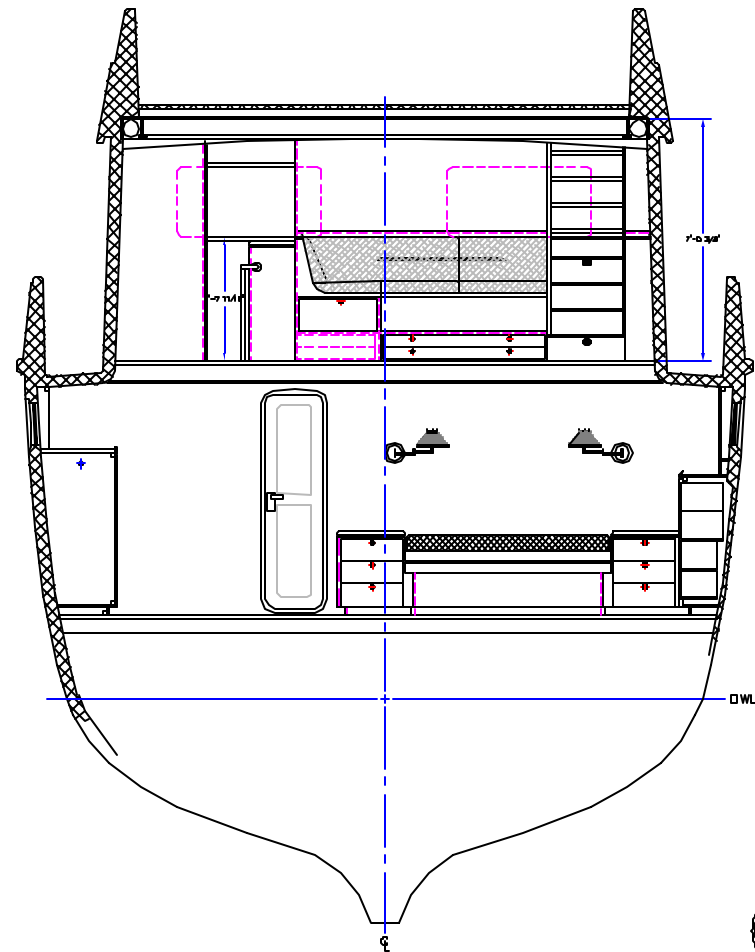
SECTION @ STATION 3.5 LOOKING AFT 1/8\"/>
