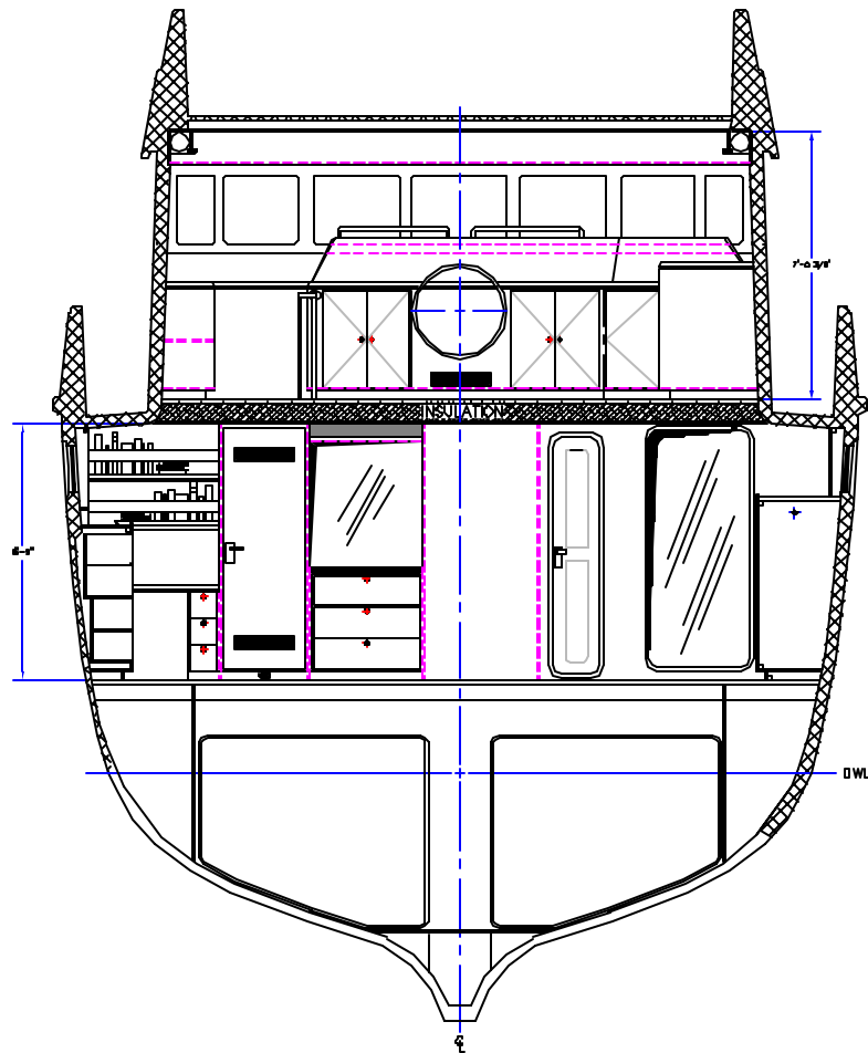
SECTION @ STATION 3.5 LOOKING FWD 1/8\"/>
