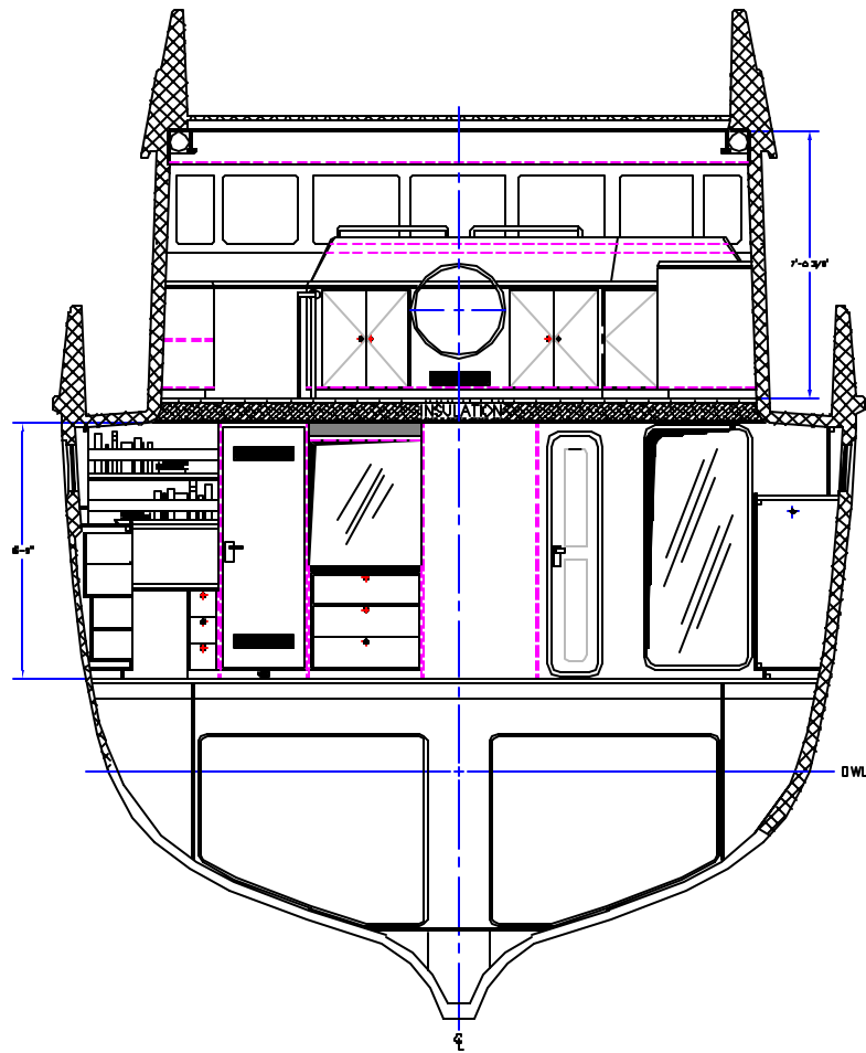
SECTION @ STATION 3.5 LOOKING FWD 1/2\"/>
