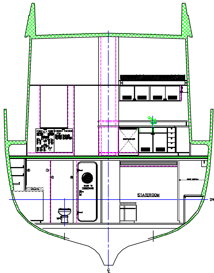
STATION 5 LOOKING AFT 1/2"=1'-0"
