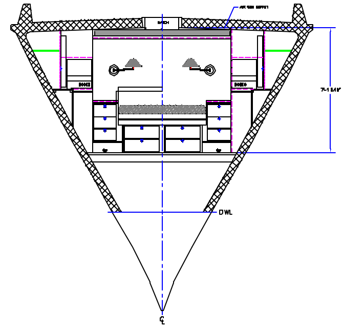
SECTION @ STATION 1 LOOKING FWD 1/2\"/>
