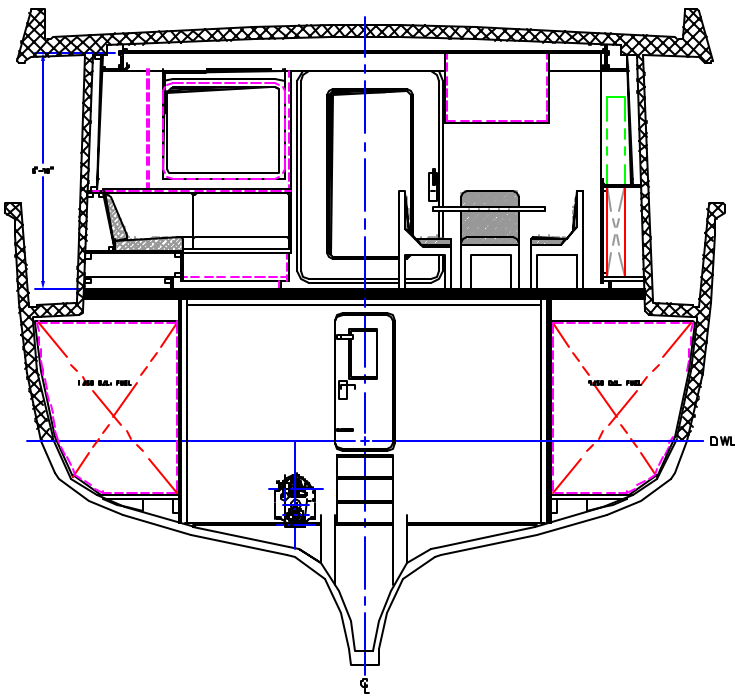
SECTION @ STATION 7 LOOKING AFT 1/2\"/>
