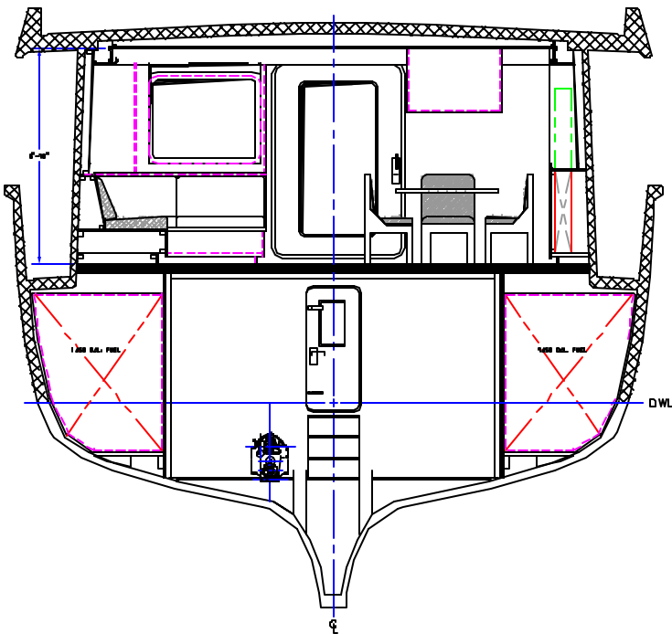
SECTION @ STATION 7 LOOKING AFT 1/8\"/>
