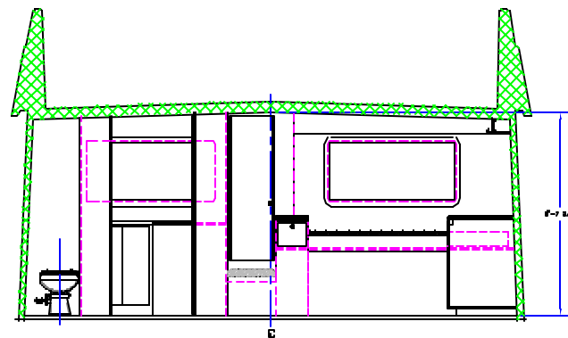
STATION 5 LOOKING AFT 1/2"=1'-0"
