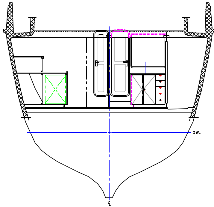
SECTION @ STATION 2.75 LOOKING FWD 1/2\"/>
