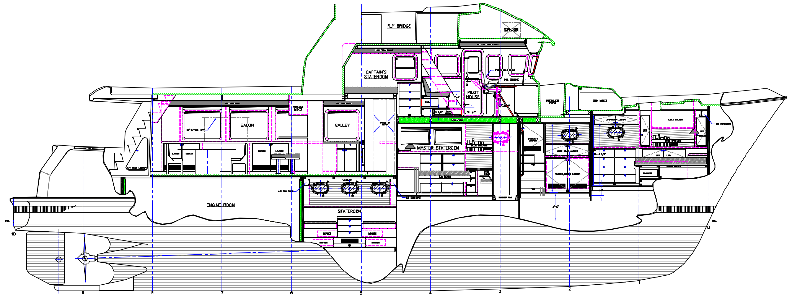
PORT INTERIOR PROFILE SECTION 1/2"=1'-0"
