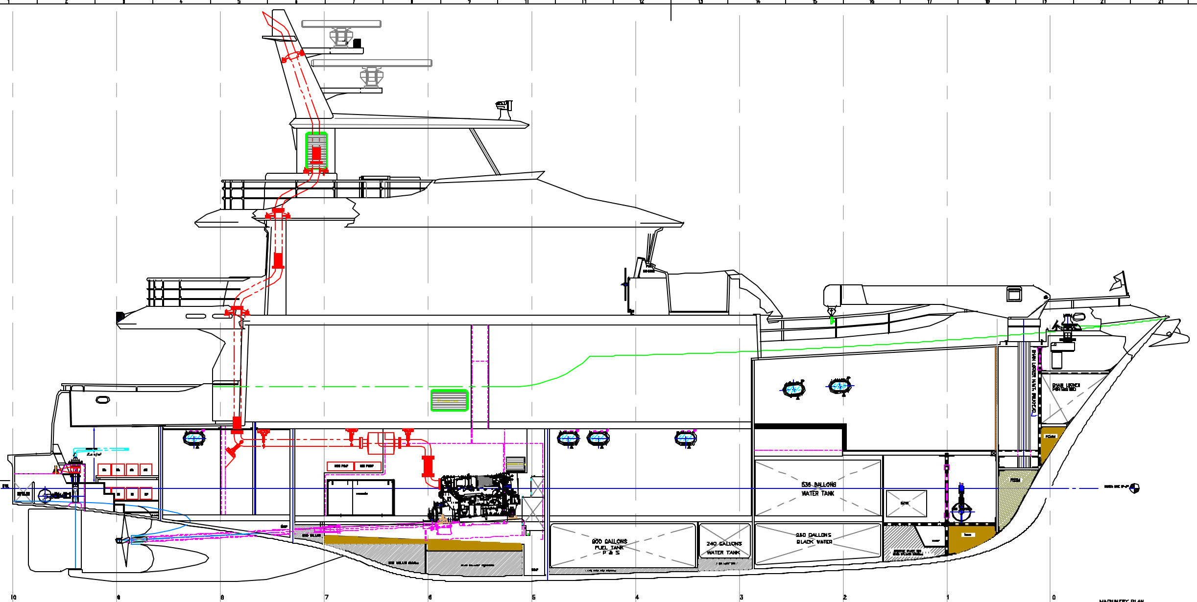
MACHINERY PLAN 86-7-2
